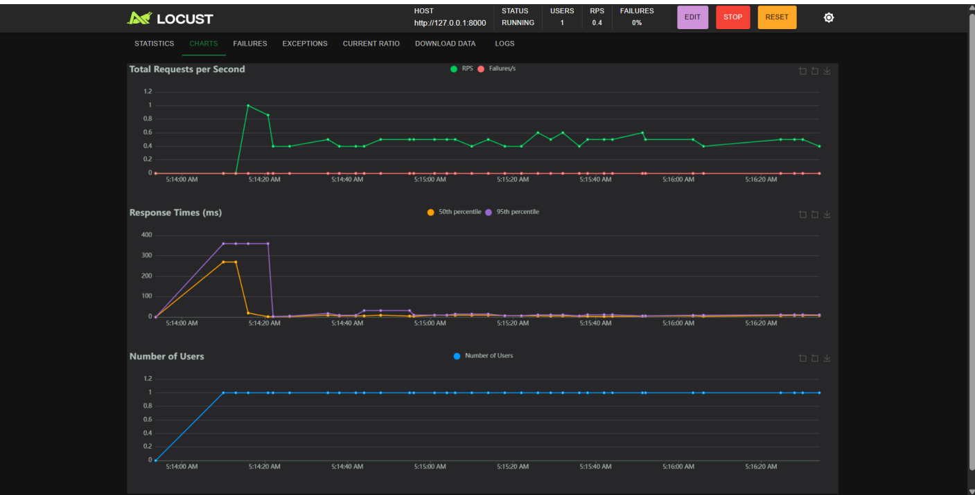
Charts screenshot: requests per second, response time percentiles, and number of users.
