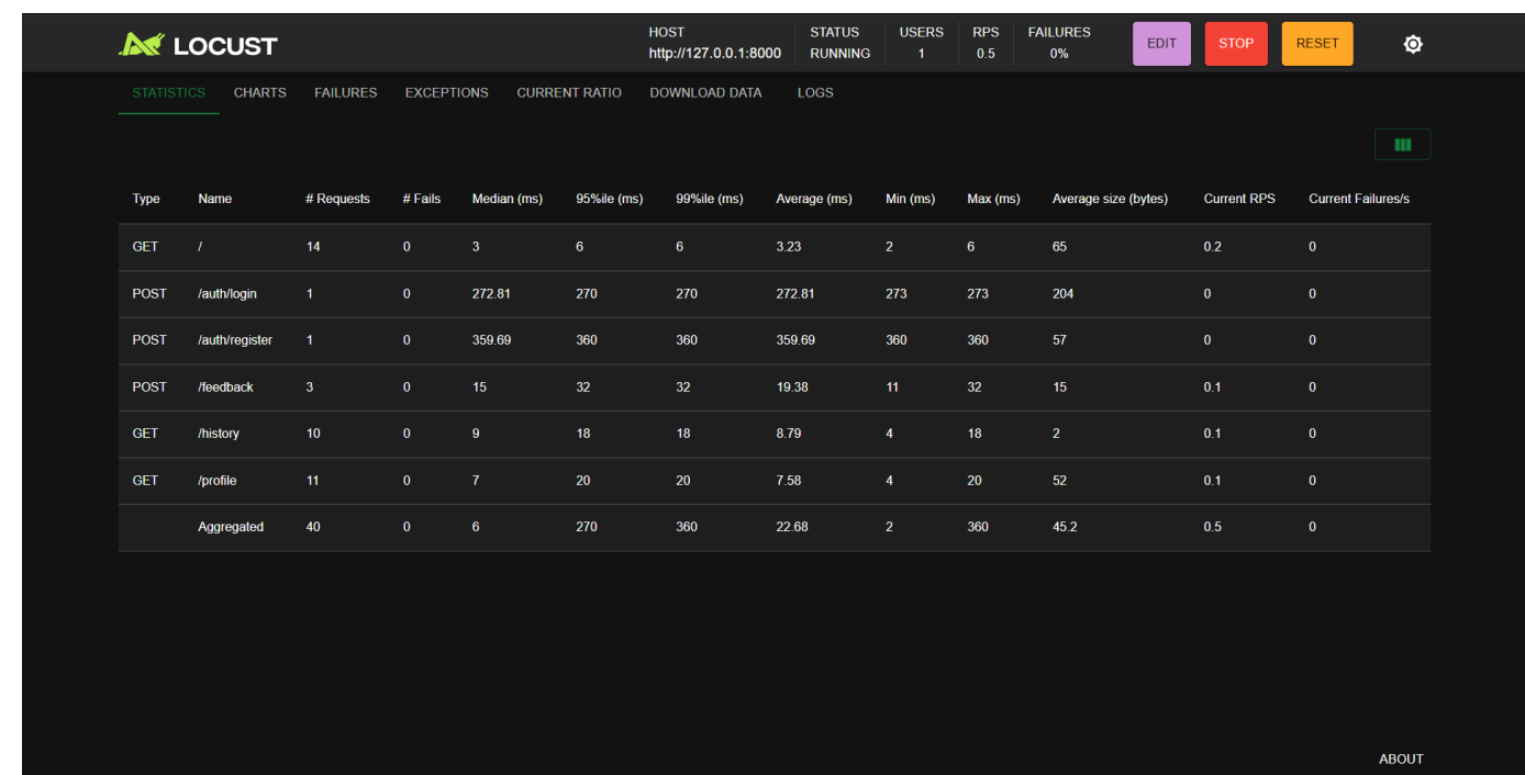
Statistics screenshot: endpoint rows, aggregate totals, response times, failures, and current RPS.
